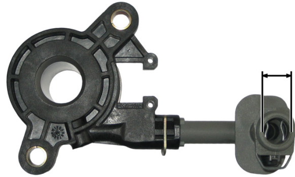
Fig. 2: CSC 3182 600 129 → 3182 654 146 → 3182 654 299 Hydraulic connection diameter: 13.3 mm
