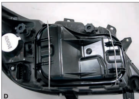
D Mount the cover and engage the spring.
