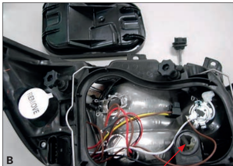
B Remove the reflector bracket.
