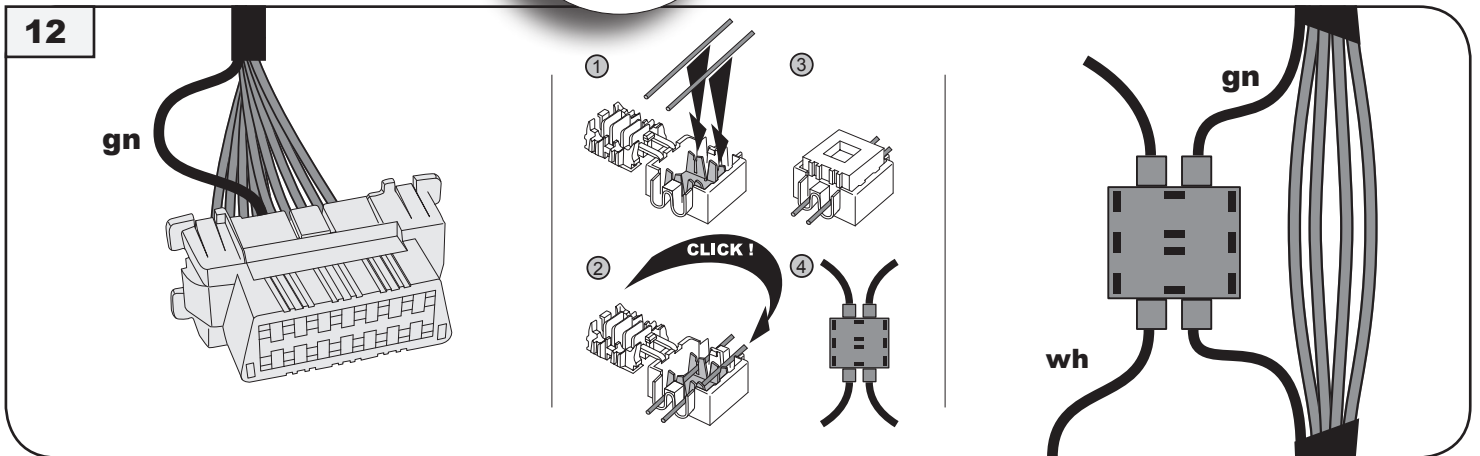
kabel gn (CAN) Fahrzeug PIN 16 cabel gn (CAN) car PIN 16
